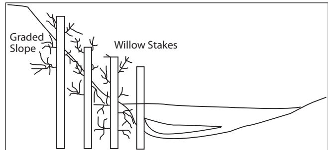
Figure 2. Willow post installed below depth of water table and streambed scour.
